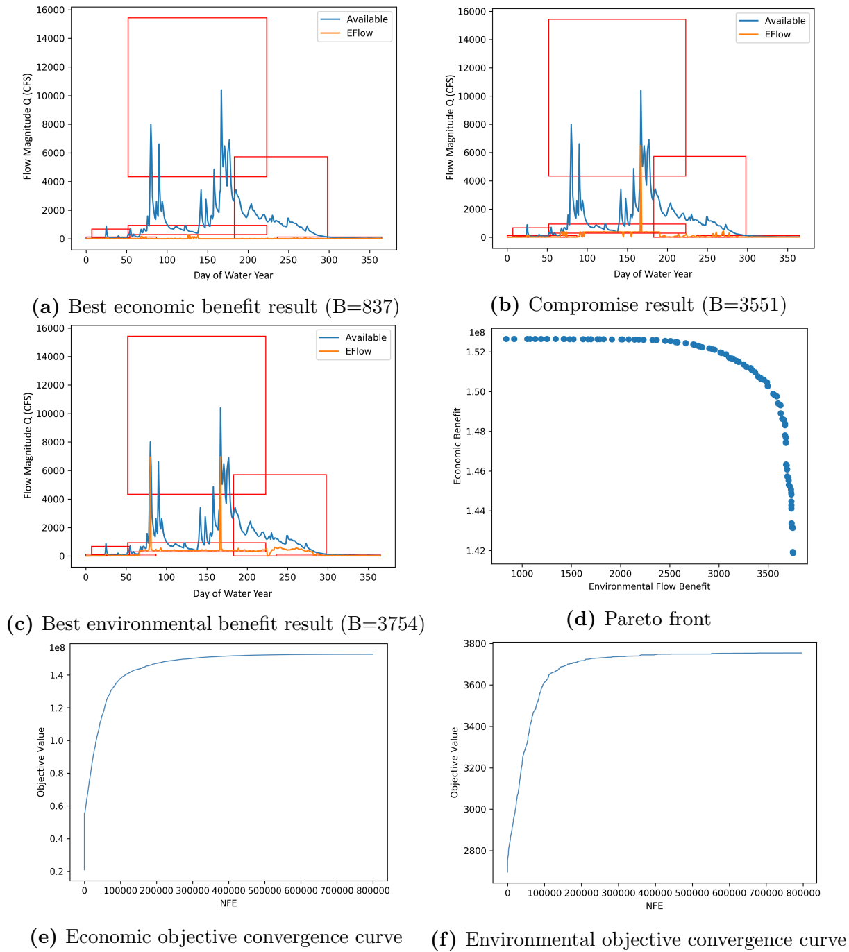
Figure 4.3 Results of Model E for the Michigan Bar stream segment for water year 2011 with random seed 912264360. Red boxes on plots show outer bounds of constructed flow components. Convergence plots show best objective value encountered at each NFE. Full convergence plots are in Figure C.13 and Figure C.14 .
