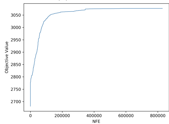
(f) Environmental objective convergence curve
